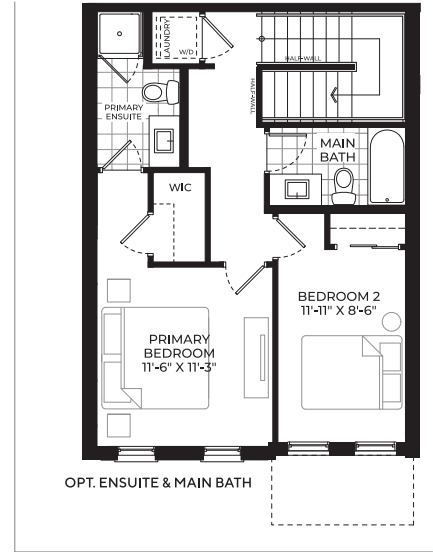
UNIT #7 (PARKING SIDE ENTRY)
