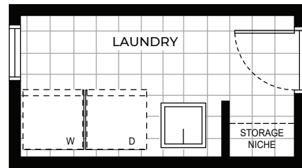
OPT. LAUNDRY LAYOUT
