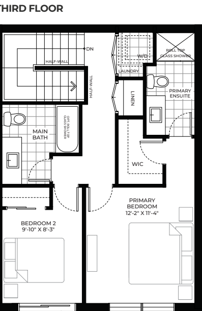
ELEV E - INTERIOR 1,436 SQ. FT. 2-BED, 2.5-BATH
