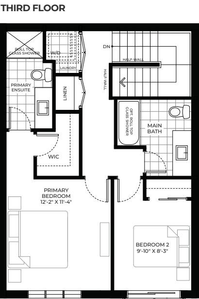
ELEV D - INTERIOR 1,457 SQ. FT. 2-BED, 2.5-BATH
