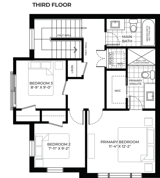
CORNER ELEV 1,677 SQ. FT. 3-BED, 2.5-BATH
