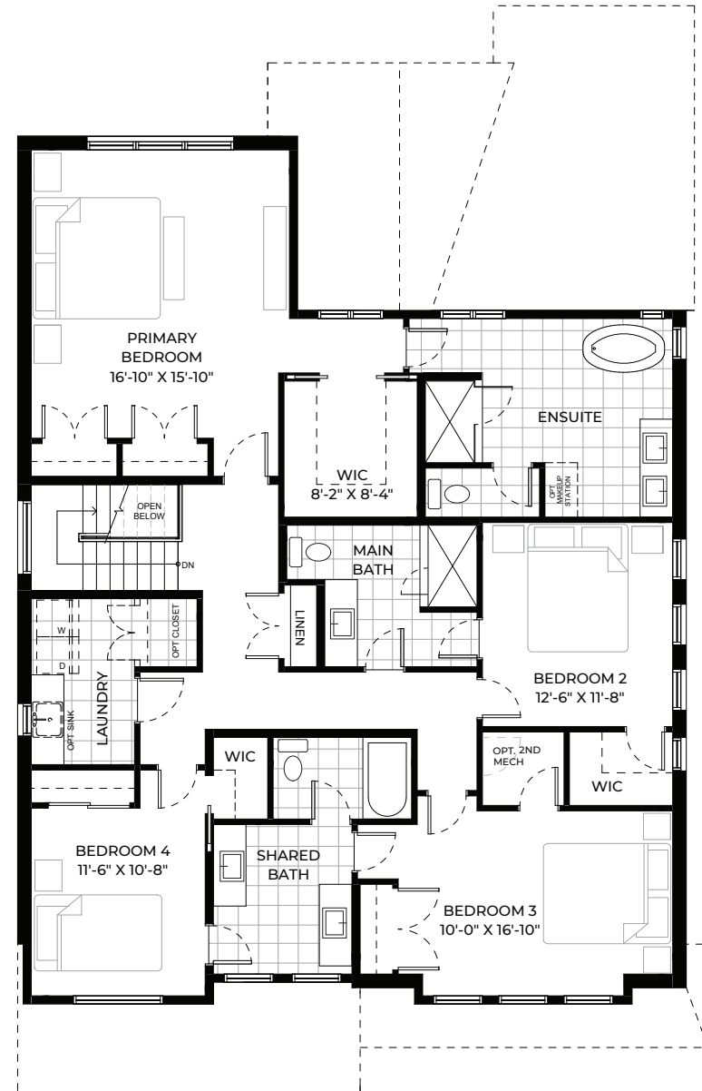
SECOND FLOOR
