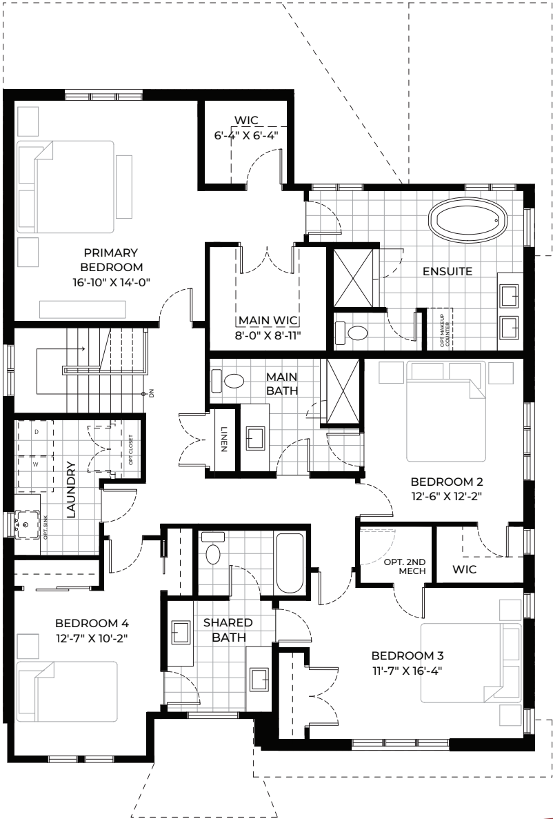
SECOND FLOOR
