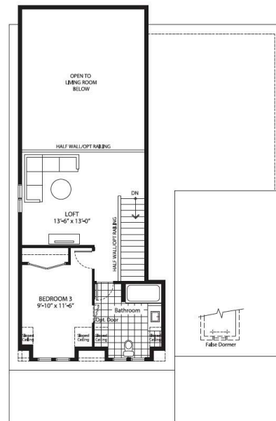
LOFT ELEVATION A
