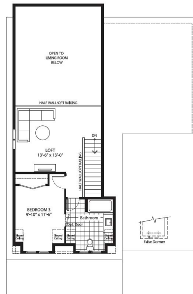
LOFT ELEVATION A
