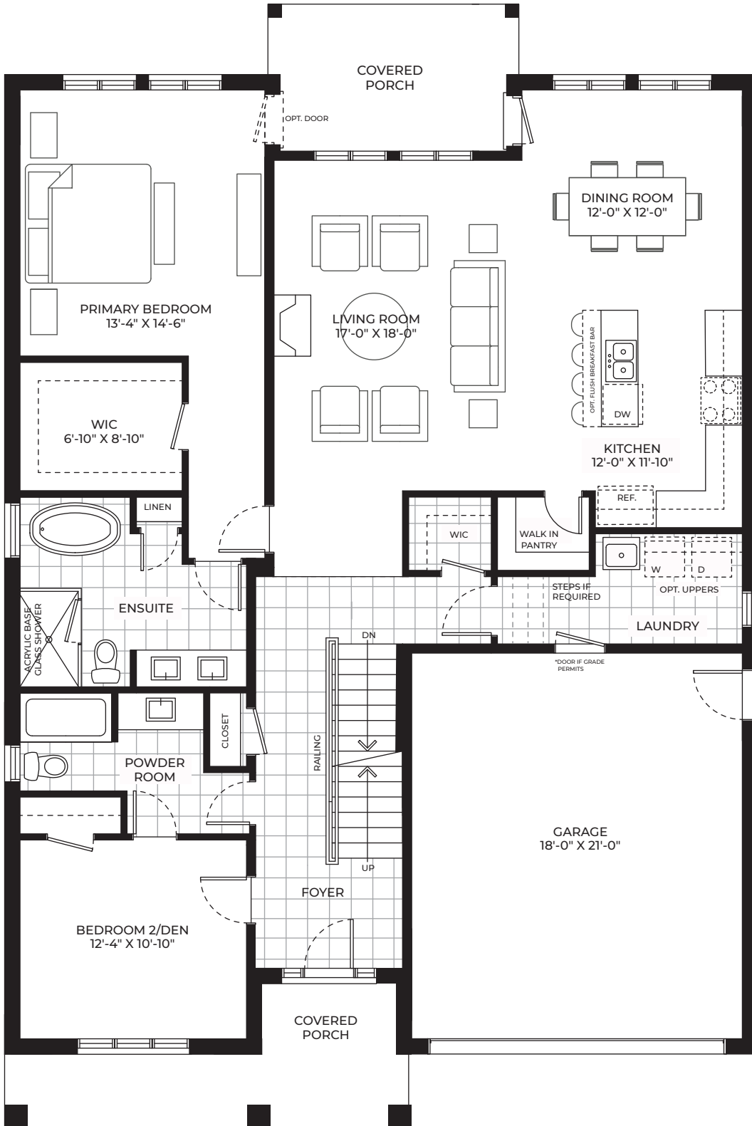
OPTION A - NOOK OPTION B - LINEN (Upgrade)
