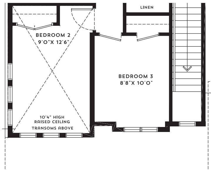
▶ SECOND LEVEL ELEVATION A*
